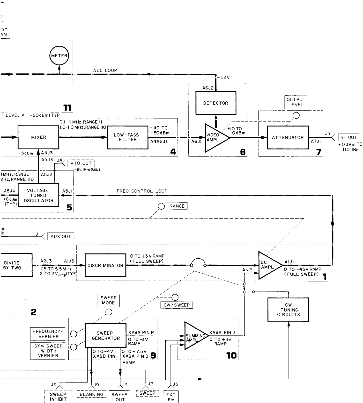
Figure 8-4. Detailed Block Diagram
