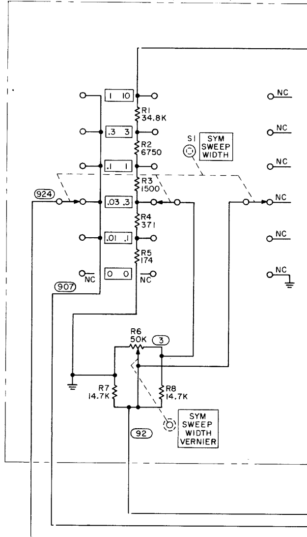
A11 SYM SWEEP WIDTH SWITCH ASSY (08601-6010)
