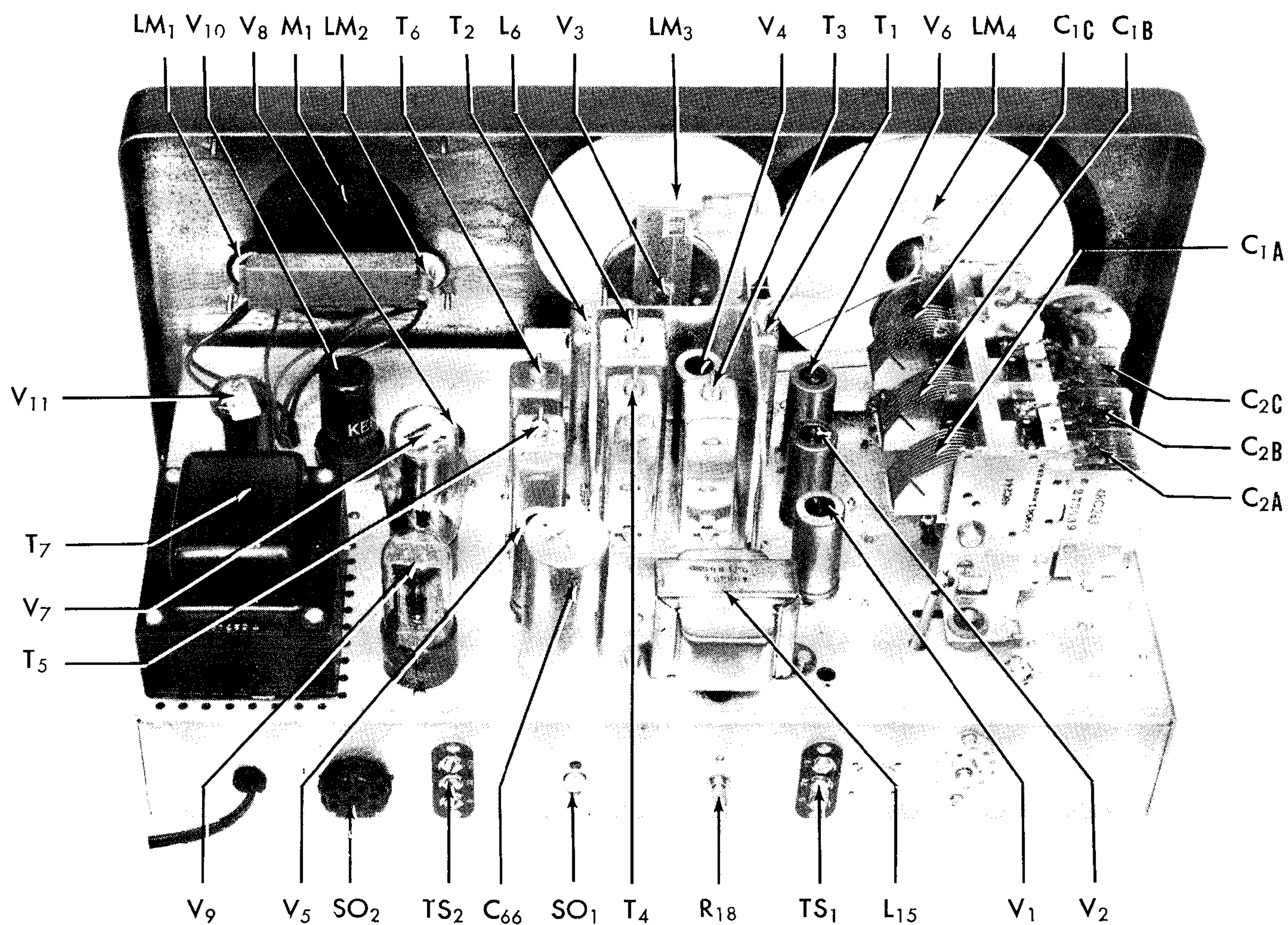
FIG. 5 TOP VIEW - COMPONENT LOCATION
