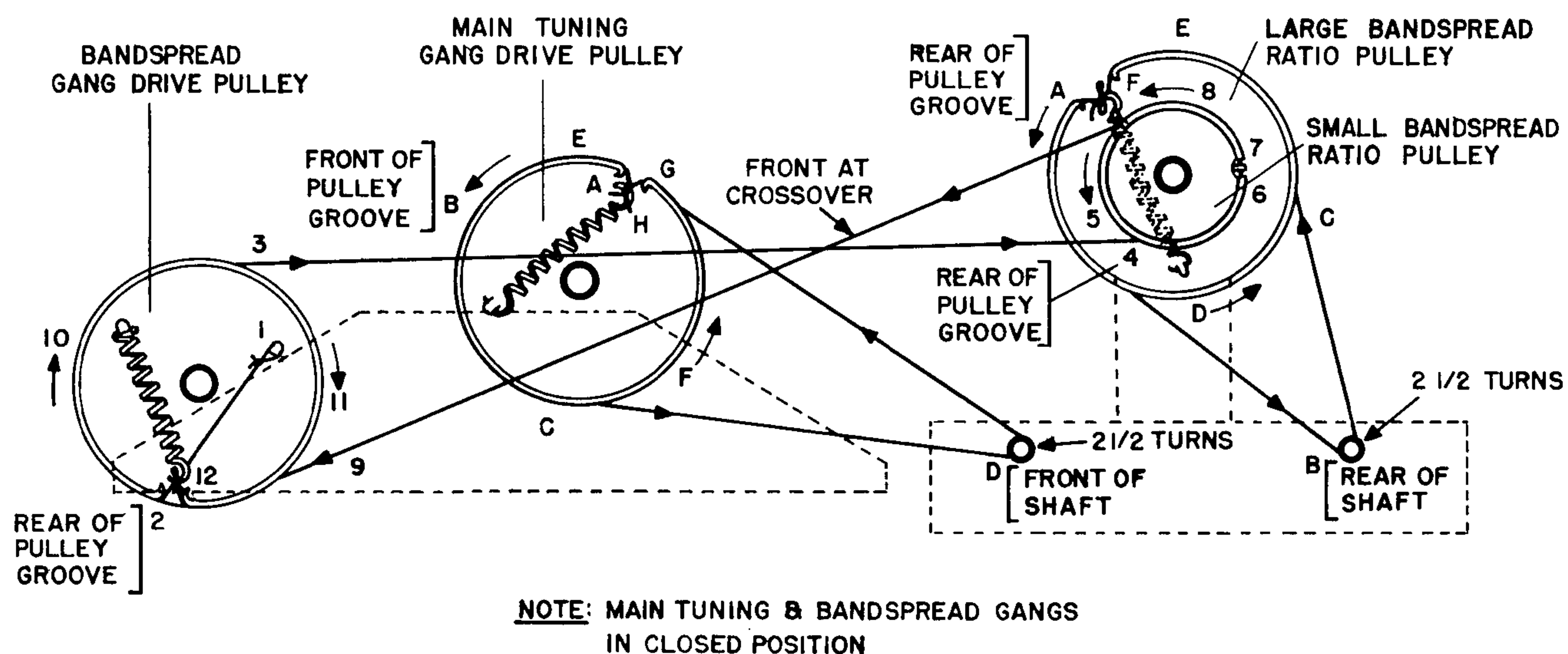
FIG. 2. DIAL CORD STRINGING PROCEDURE
