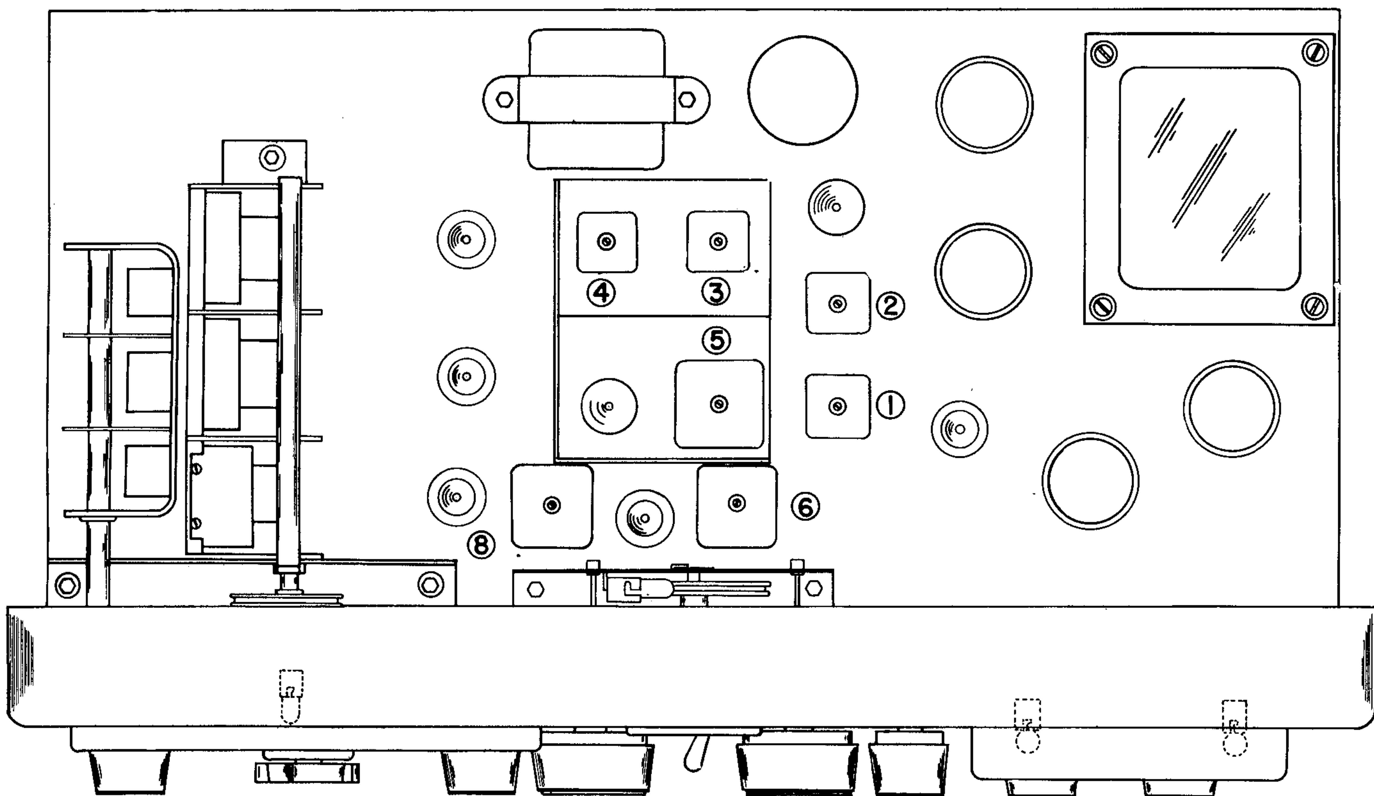
FIG. 3 TOP VIEW - LOCATION OF ALIGNMENT ADJUSTMENTS
