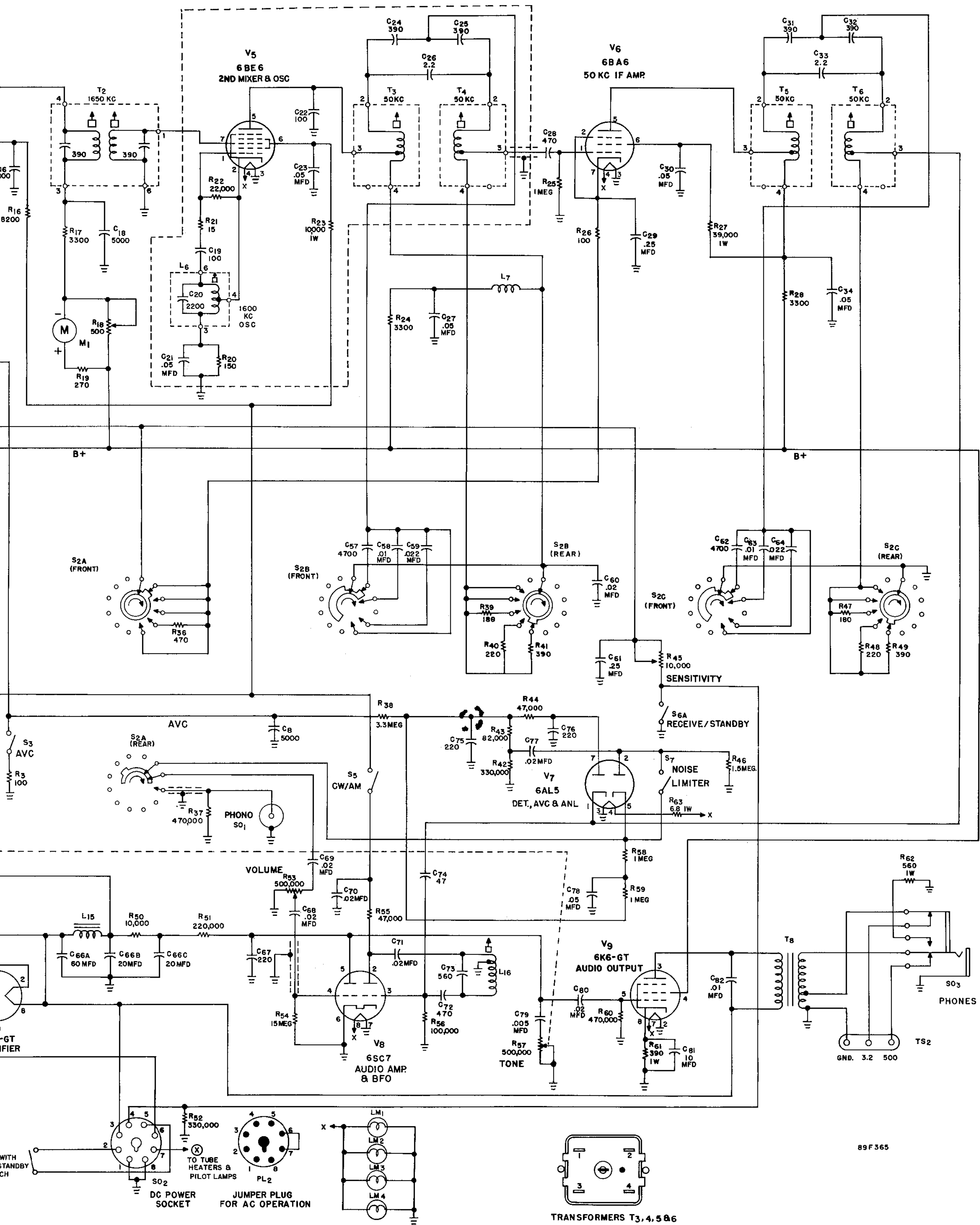
FIG. 10 SCHEMATIC DIAGRAM
