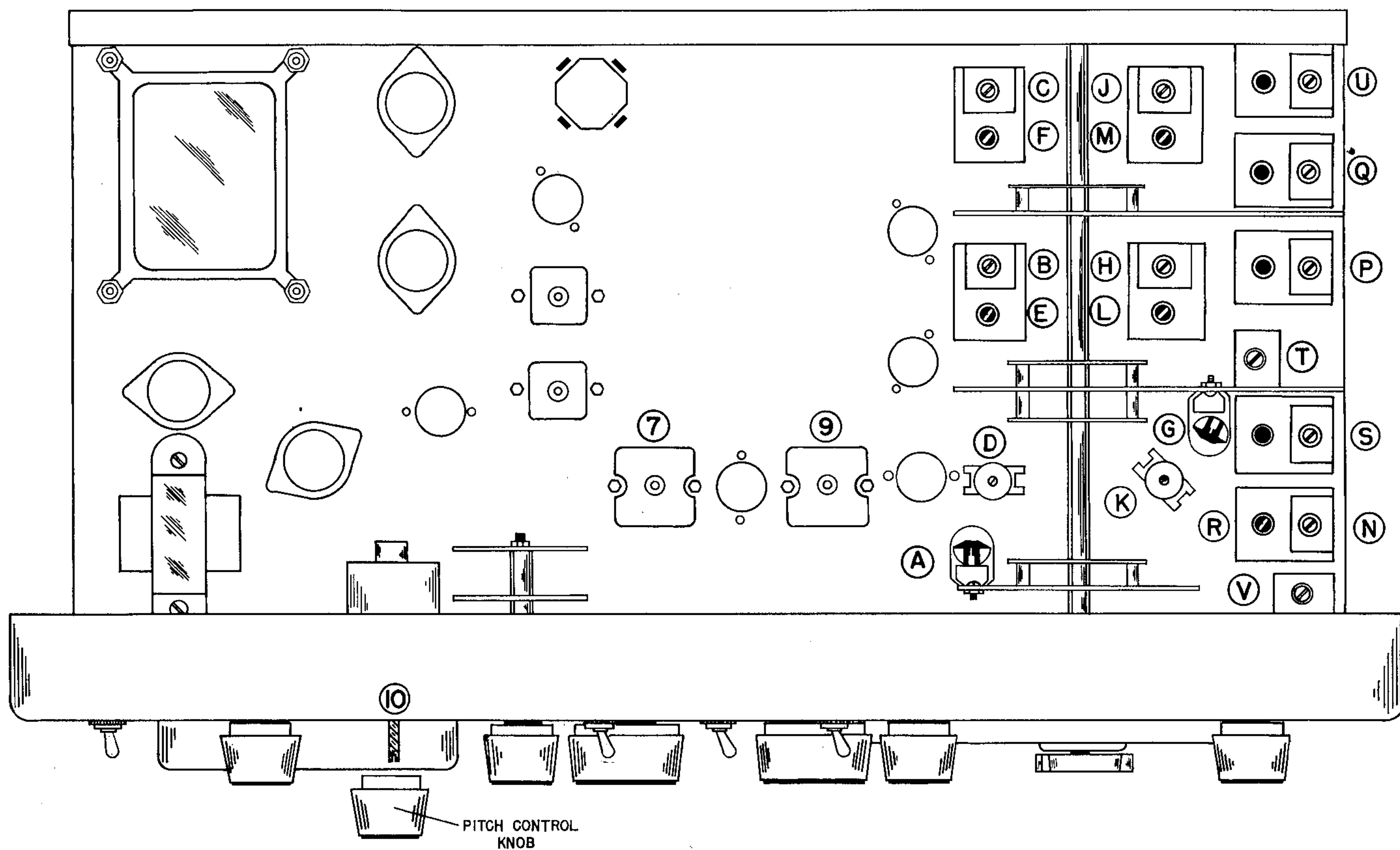
FIG. 4 BOTTOM VIEW - LOCATION OF ALIGNMENT ADJUSTMENTS
