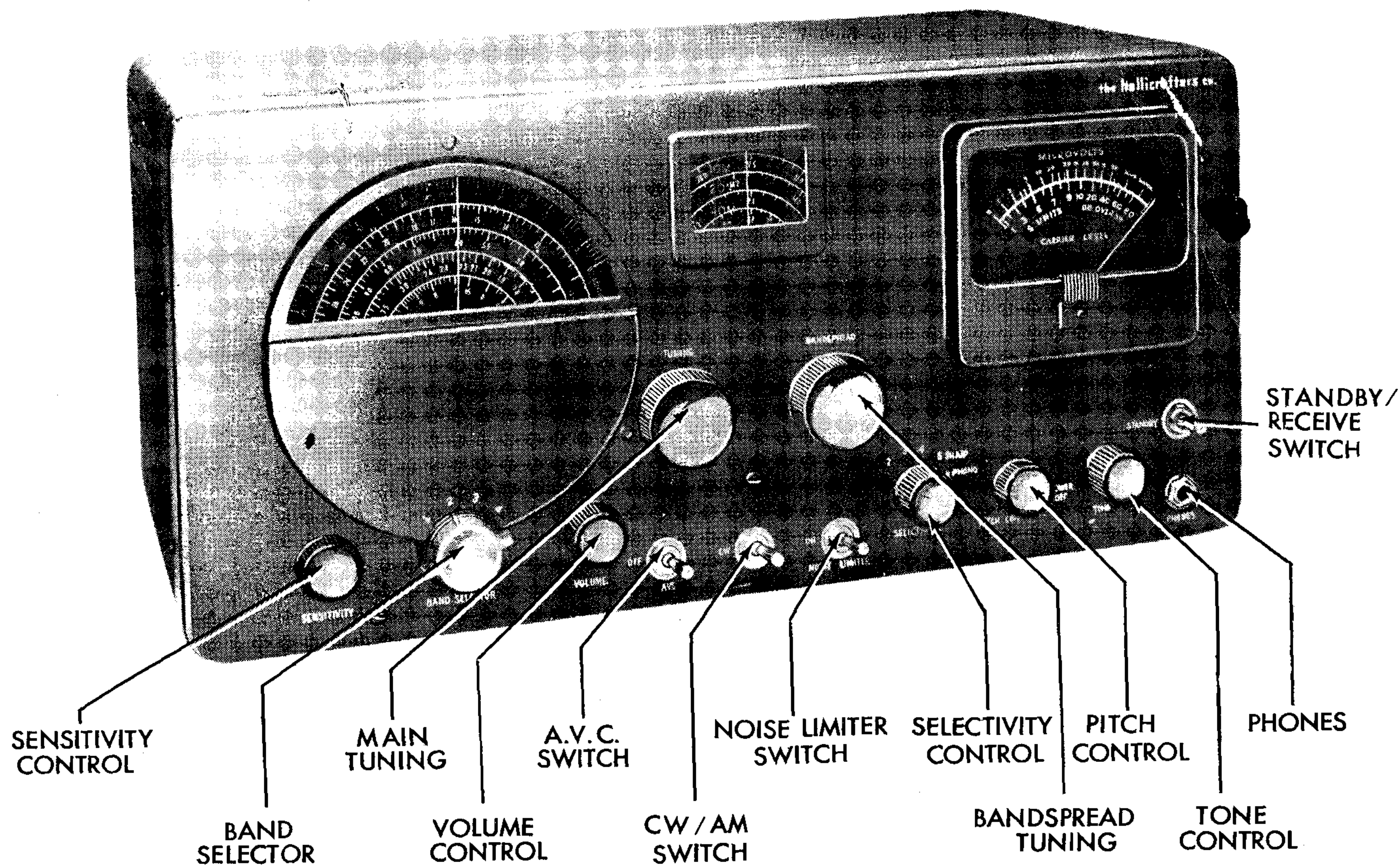
FIG. 1. COMMUNICATIONS RECEIVER MODEL S-76
