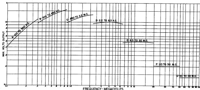
Figure 5.3 - Maximum Voltage Output
