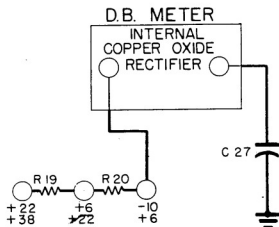
Figure 2.9 - Decibel Meter
