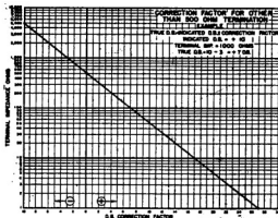
Figure 3.3- Correction Factor for Other Than 500 Ohm Termination
