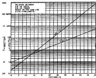
Figure 3.2 - DB-Voltage Conversion Chart
