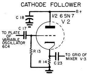
Figure 2.3 - Cathode Follower
