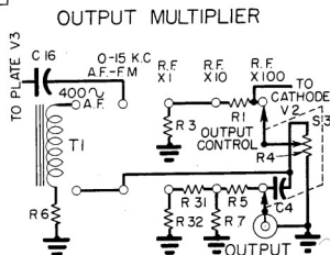
Figure 2.8 - Output Multiplier
