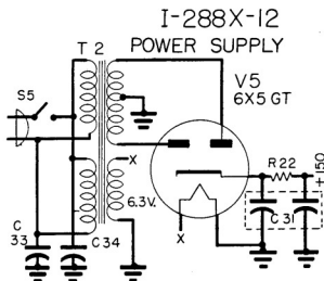
Figure 2.1 - Power Supply
