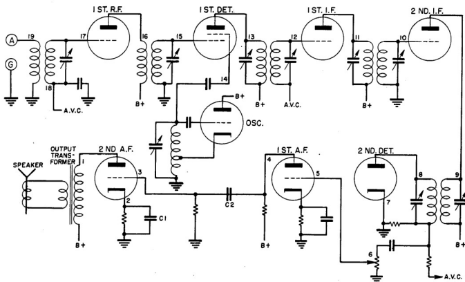
Figure 4.1 - Basic Circuit, Superheterodyne Receiver
