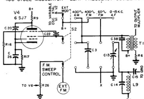
Figure 2.4 - 400 Modulator - Beat Frequency Oscillator
