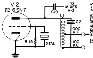
Figure 2.7 – Crystal Oscillator
