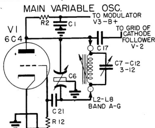
Figure 2.2 - RF Main Variable Oscillator
