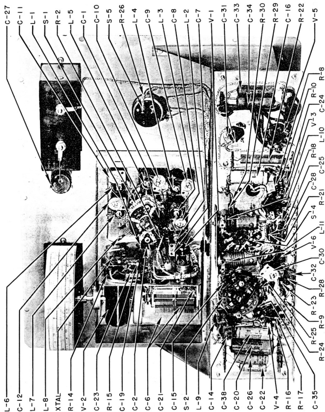
Figure 5.1 - Model 288X, Case Removed, Rear View
