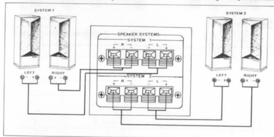
Figure 5. Speaker System Connections
