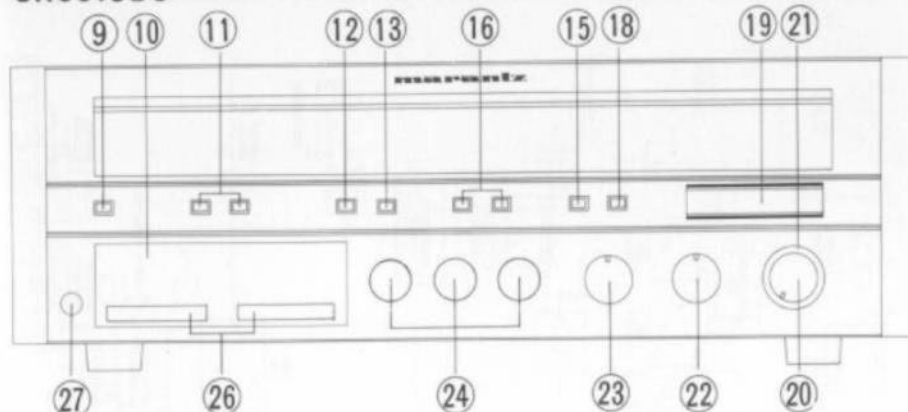
Figure 7. Front Panel
