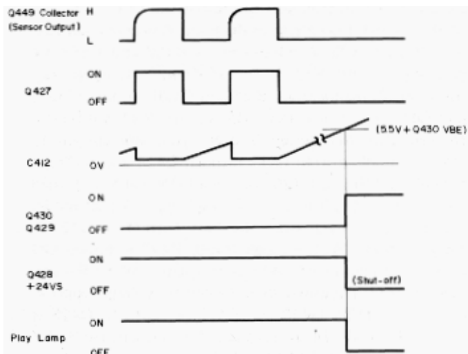
Fig. 2.3.6 Timing Chart
