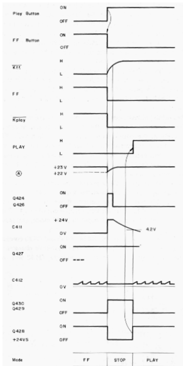
Fig. 2.3.7 Timing Chart
