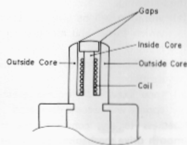
Fig. 2.1.3 Sectional View of Erase Head
