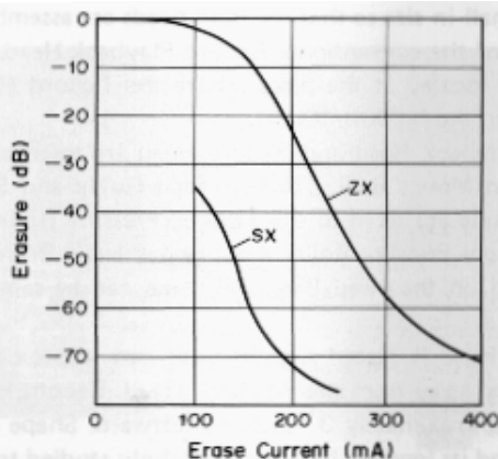
Fig. 2.1.4 Characteristics of Erasing Current and Erasure
