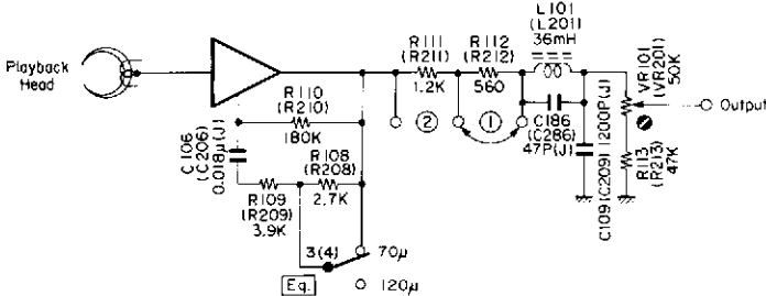
Fig. 7.8 Playback Amp.
