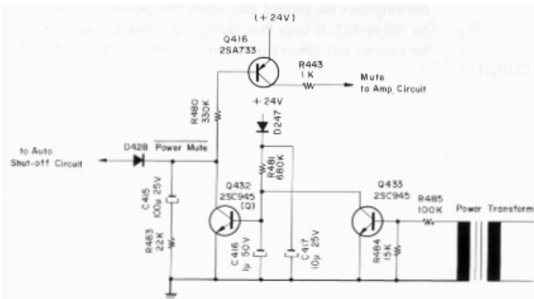
Fig. 2.3.3 Power-mute Circuit
