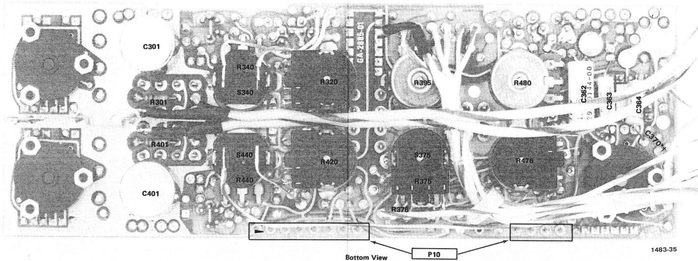
Fig. 9-1B. A1 Input Board Front View (top) and Back View (bottom). Below SN B100000.
