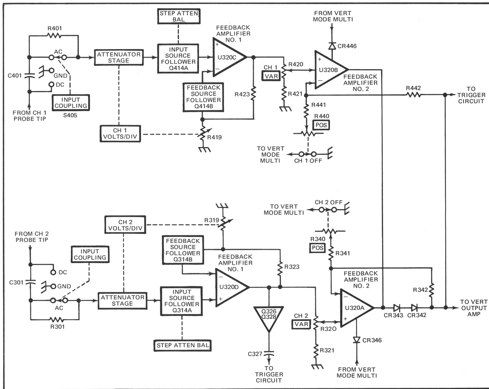
Fig. 6-1. Vertical input amplifiers detailed block diagram.
