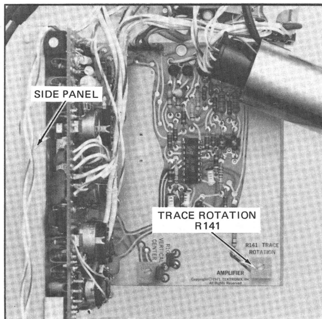
Fig. 4-3. Location of Trace Rotation adjustment.
