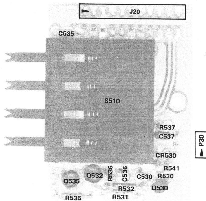
Fig. 9-4. A4 Single Sweep Board. 1483-38
