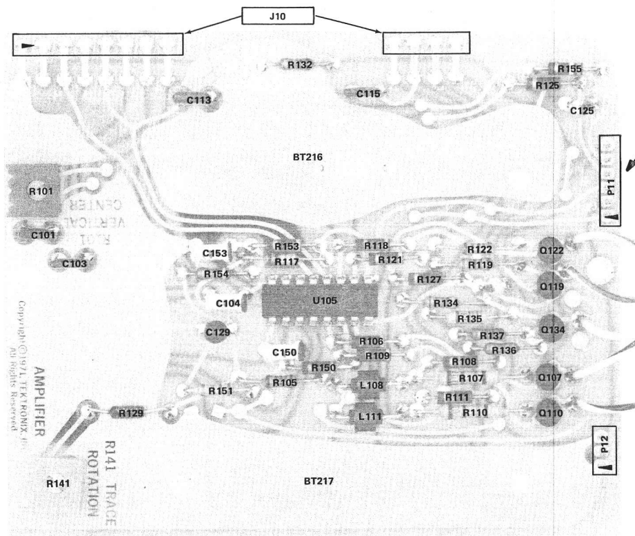
Fig. 9-2. A2 Amplifier Board
