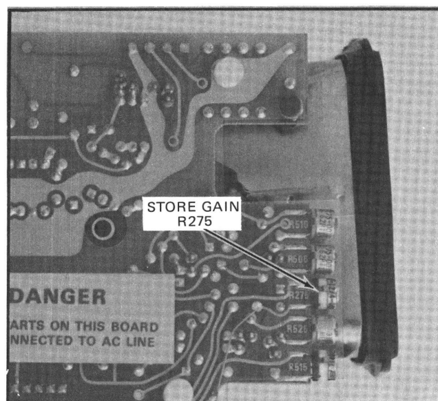
Fig. 4-7. Location of Store Gain adjustment.
