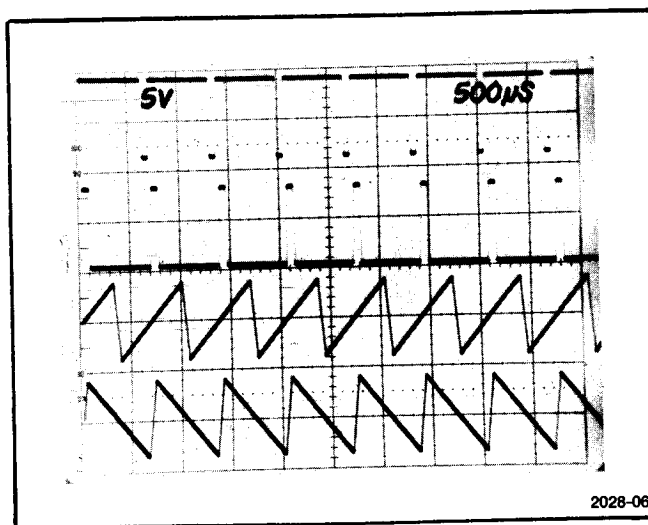
Fig. 2-8. RAMPS AND PULSES. These are obtained from the basic waveforms by using the SYMMETRY control.
