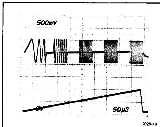
Fig. 2-21. TONE BURST TESTING. The lower trace is the linear ramp from the LIN SWEEP OUTPUT terminal.
