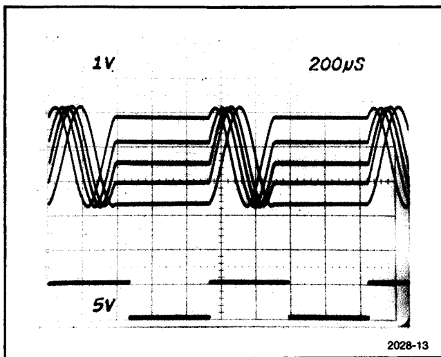
Fig. 2-15. PHASE CONTROL OPERATION. This photograph illustrates PHASE control usage in the triggered mode. The five super-imposed traces illustrate the effect of the phase control. This control provides approximately \pm 80^\circ of shift. The bottom trace is the triggering waveform.
