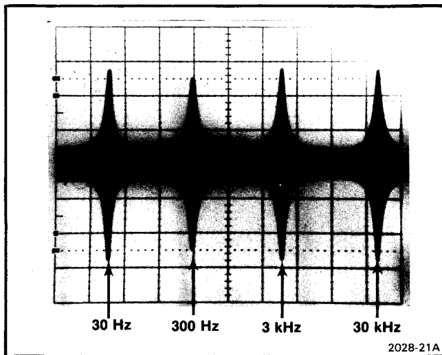
Fig. 2-23. Logarithmic sweep showing even spacings of filter output frequencies.
