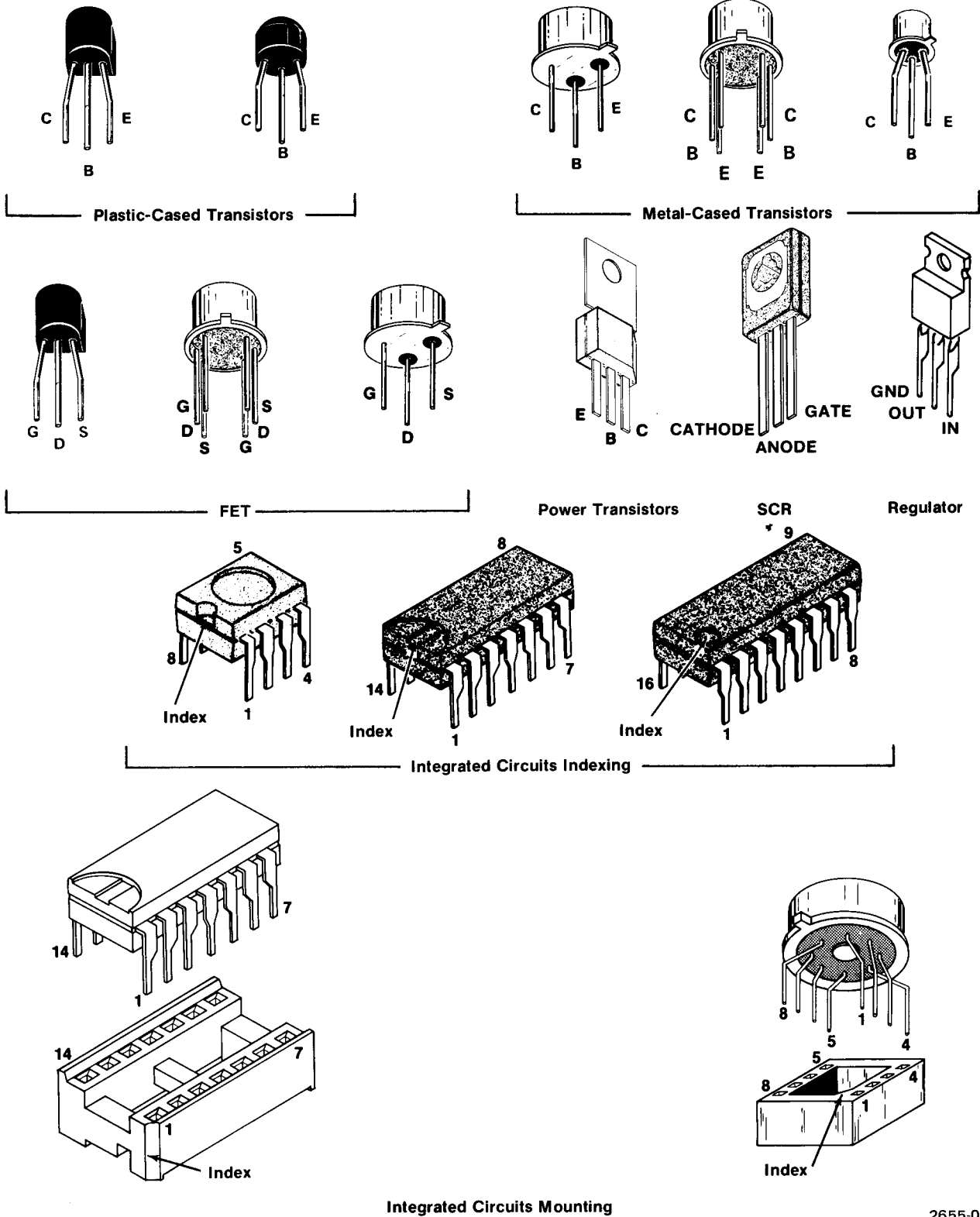
Fig. 8-1. Semiconductor basing.
