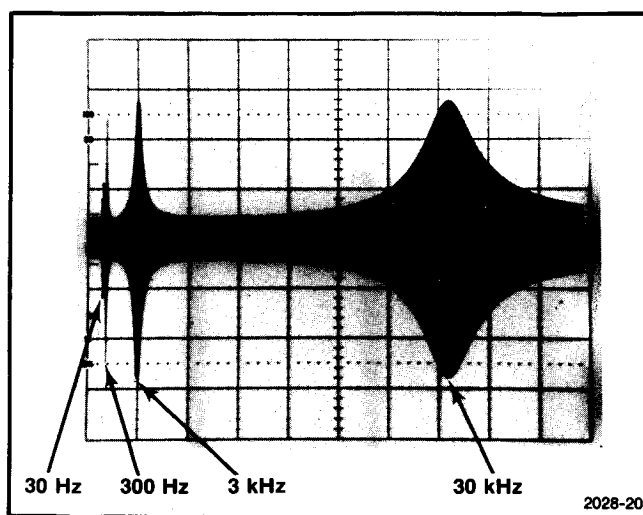
Fig. 2-22. Linear sweep showing skewed spacing of filter output frequencies.
