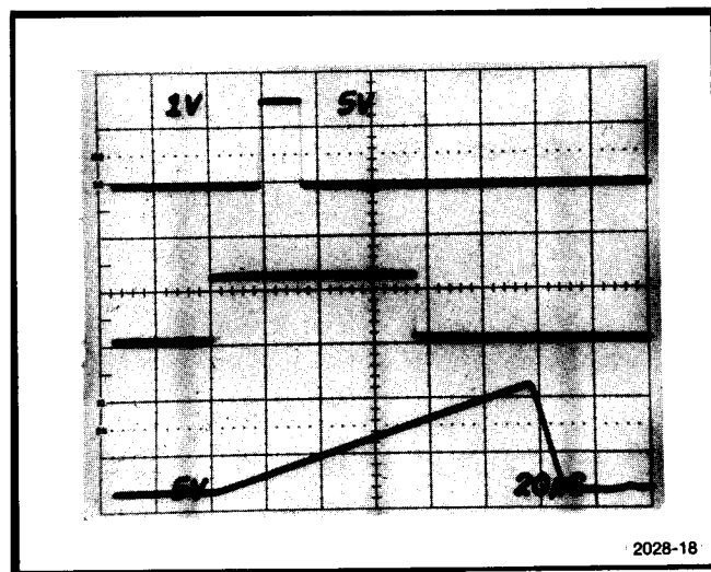
Fig. 2-20. DELAYED OPERATION. A wide range of delay times are available by using the internal sweep generator as a delay generator. The middle trace is the underlayed input signal applied to the SWEEP TRIG INPUT. The bottom trace is at the LIN SWP OUT connector. This ramp is applied to the external trigger INPUT connector. The top trace is the delayed output pulse. The amount of delay is proportional to the sweep duration and the setting of the TRIG LEVEL control. Be sure when using the sweep as a delay generator to set the STOP FREQ dial fully ccw.
