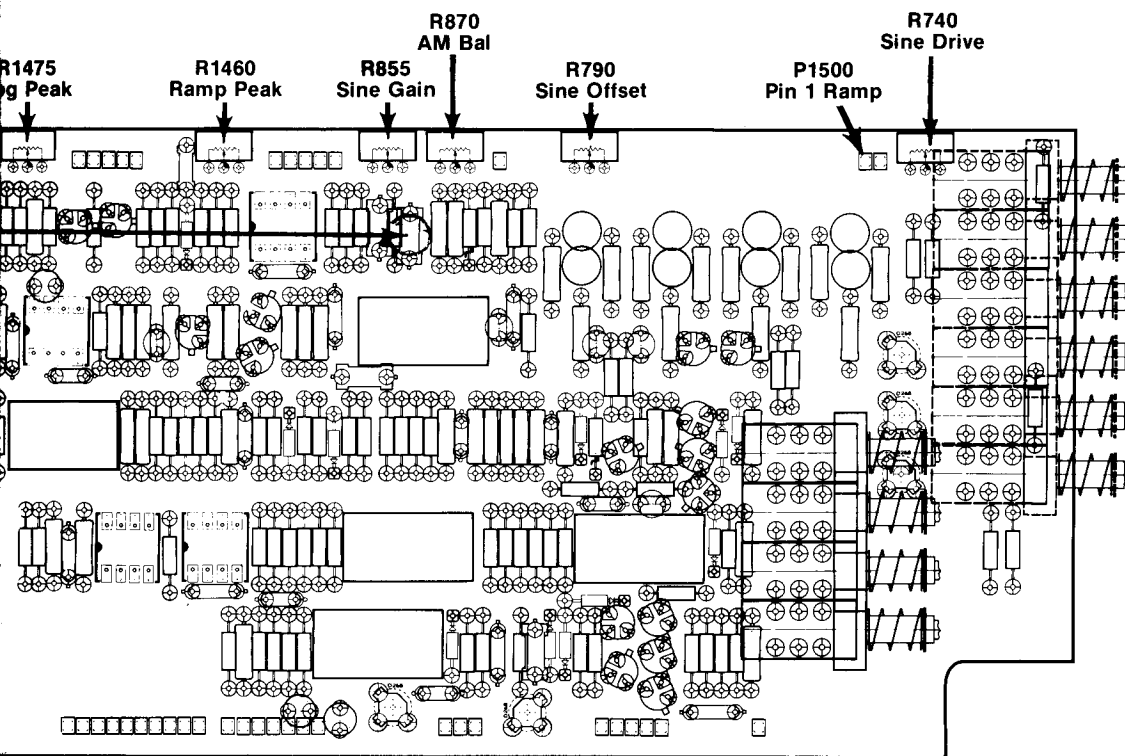
A2 Function Board
