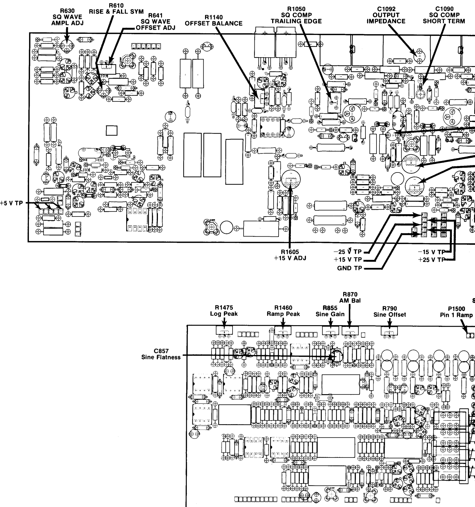
Fig. 8-2. Adjustment locations.
