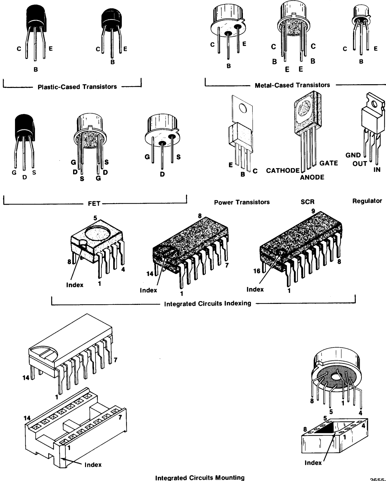
Fig. 5-1. Semiconductor Basing.
